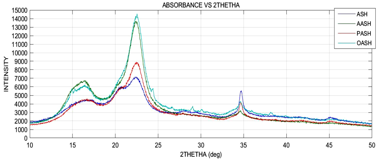
Fig. 2 XRD Pattern of Acid/Alkali Treated Soya-hulls
