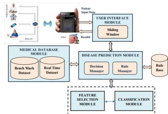
Figure 3.1 Architecture of Proposed Disease Prediction System
