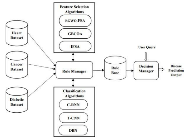
Figure 3.2 Workflow of Proposed Disease Prediction System
