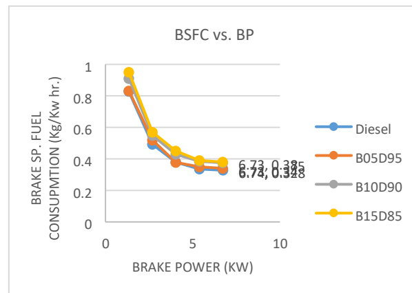
Figure 7 BSFC Vs BP graph
