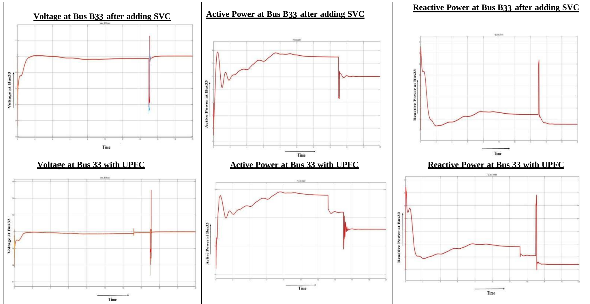
Fig.10 Results obtained after Running the simulation model for all the three FACT devices (i) with STATCOM (ii) With SVC (iii) with UPFC for Examining their Behaviour under Normal and Faulty Conditions [ the voltage profile ,Active Power and Reactive Power Compensation is Examined in MATLAB, the fault L-L-G is subjected at 15 seconds and at 15.1 second it was removed so the above results are for that durational behaviour of FACT device for Ratedi Site ,WEC E-31 Convertor wind FARMS]
