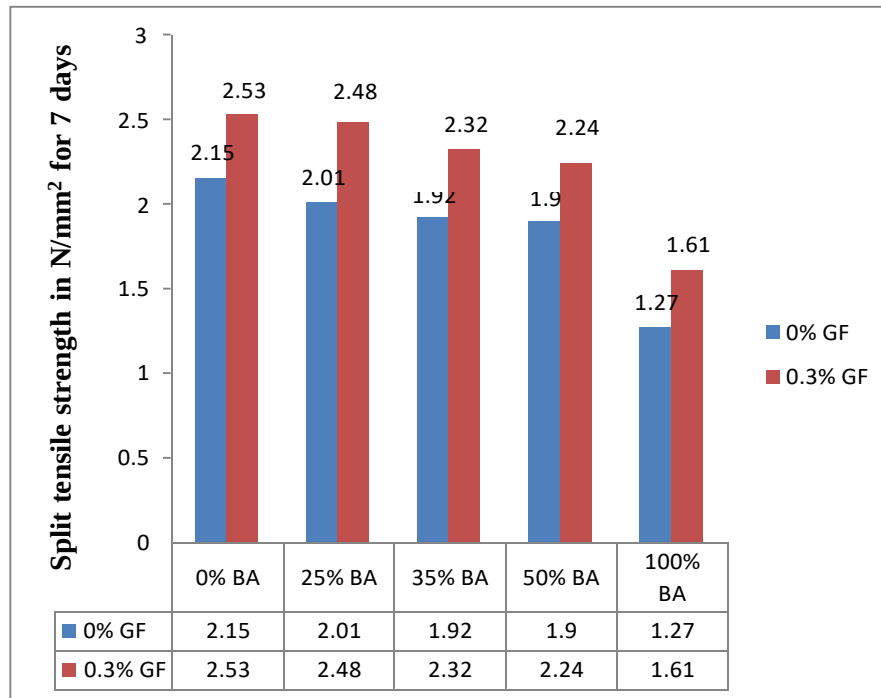
Fig. 8.3 Split Tensile Strength Results in N/mm 2 for 7 days
