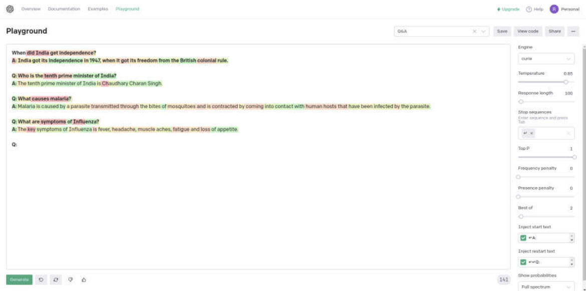
Fig 2.6 GPT-3 playground
