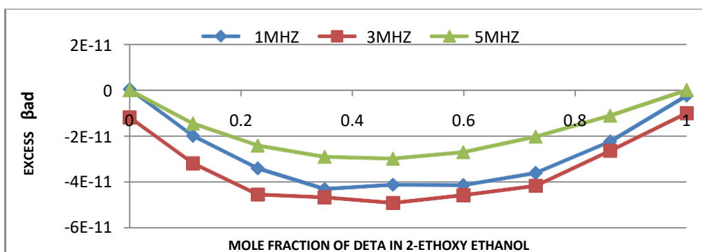
Fig 10 Graph between variation of excess adiabatic compressibility & mole fraction of DETA in 2-Ethoxyethanol at constant temperature 296K and frequencies 1MHz, 3MHz & 5MHz
